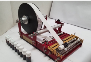
RL-RRC with Lip Balm Adapter
